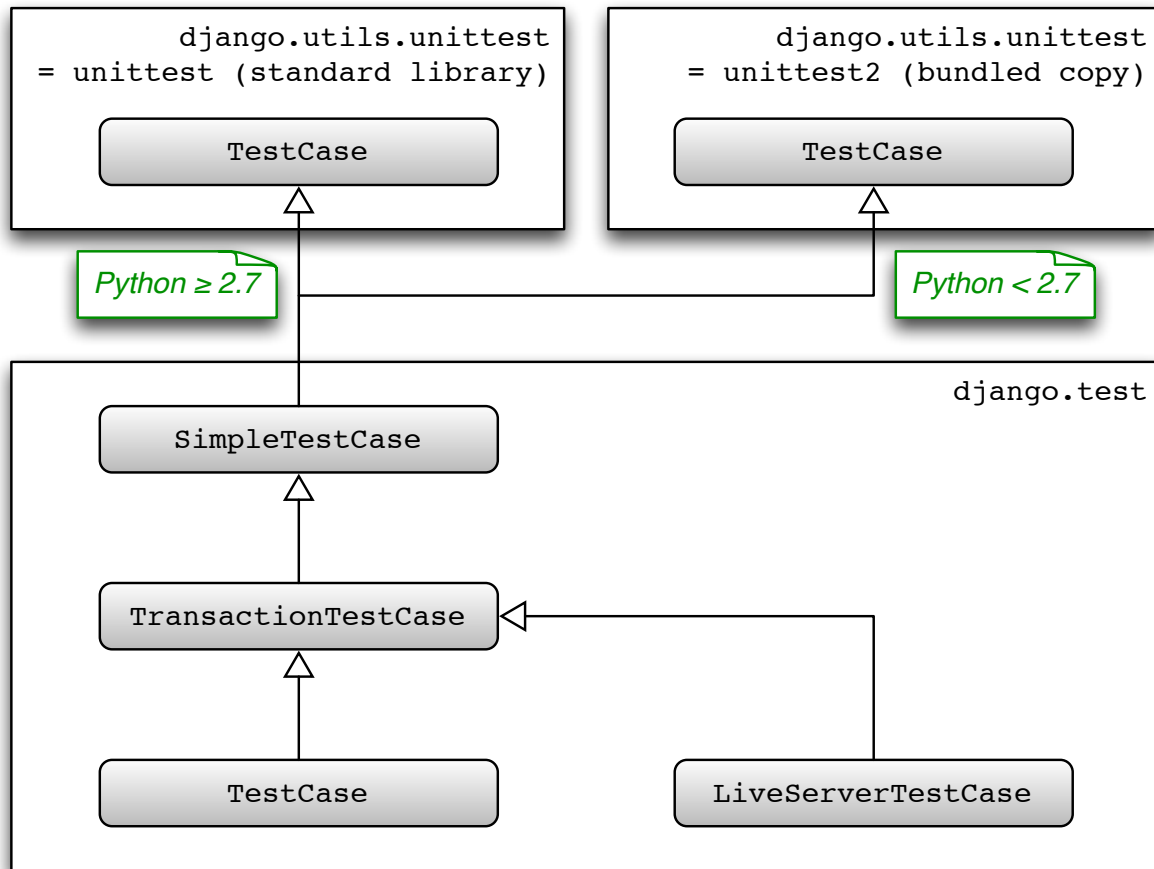
Figure 3.1: Hierarchy of Django unit testing classes
