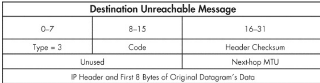
Figure 3-2. Diagram of Destination Unreachable ICMP message
