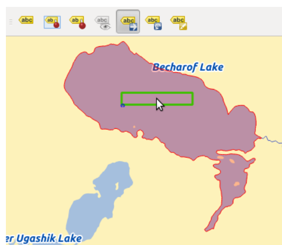
Figure 12.20: Move labels
